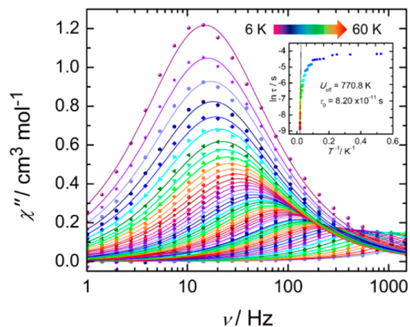
Figure 2. Frequency dependence of the \chi'' magnetic susceptibility for 1-Dy under zero applied dc field from 6 to 60 K. Solid lines represent best fits to the generalized Debye model. Inset: Relaxation time of the magnetization, \ln(\tau) vs T^{-1} ; the solid black line represents the linear fit to the Arrhenius equation.
