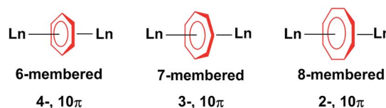
Chart 1 Ln III ions bridged by 6-, 7- and 8-membered rings.
