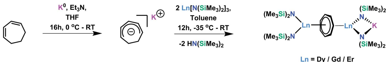
Scheme 1 Synthesis of [\text{KLn}_2(\text{C}_7\text{H}_7)(\text{N}(\text{SiMe}_3)_2)_4]^- ( \text{Ln} = \text{Dy}^{\text{III}}, \text{Gd}^{\text{III}}, \text{Er}^{\text{III}} ).
