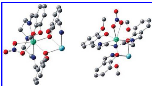
Figure 9. Two views of the structure of the calculated mononuclear lanthanide fragment of 4 . The structure of the fragments of 1–3 and 5 are similar.
