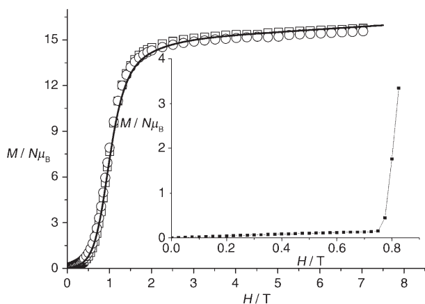
Figure 3. Molar magnetization M versus the applied magnetic field H calculated for J = -0.6 \text{ cm}^{-1} (lines) for a polycrystalline sample and the experimental powder magnetization for 1 (empty squares) and 2 (empty circles) for T = 1.8 \text{ K} . Inset: the same simulations for T = 0.1 \text{ K} .
