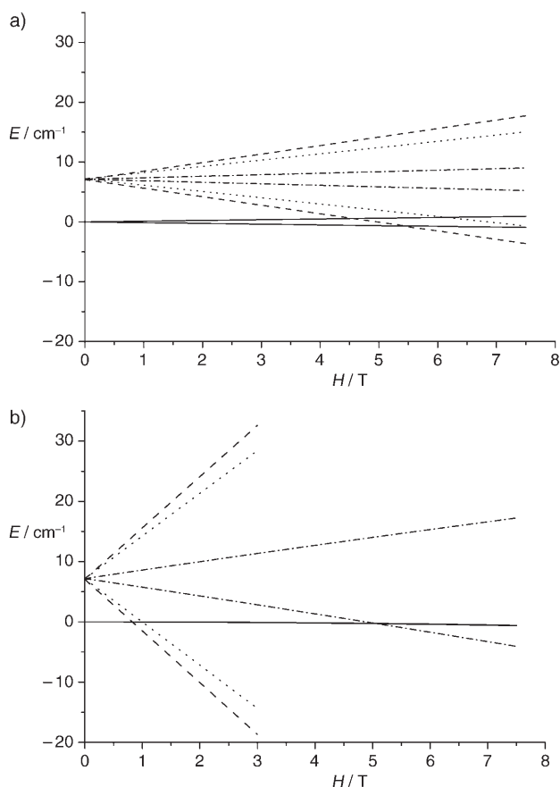
Figure 4. Evolution of the lowest magnetic states of a \text{Dy}_3 complex with applied magnetic field, simulated for J = -0.6 \text{ cm}^{-1} . a) H is perpendicular to the \text{Dy}_3 plane. b) H is applied in the \text{Dy}_3 plane.
