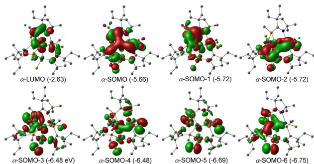
Fig. 5 Selected Kohn–Sham orbitals of the model complex [((\text{Me})(\text{Et}_2\text{-cAl})\text{P}(\text{CoCl})_3\text{O})] ( 3a' ) at the S = 3 (at UB3LYP-D3(BJ)/def2-TZVP level of theory; energies given in parentheses are in eV).
