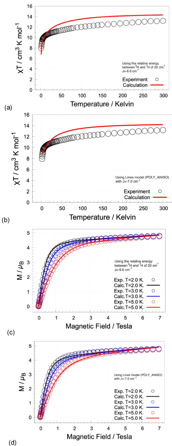
Figure 2. The \chi_M T versus T (top; H = 1 \text{ kOe} ; a–b) and M versus H (bottom; c–d) plots of complex 1·tol. Comparison between calculated and measured magnetic susceptibility (a, b) and molar magnetization (c, d) of 1·tol, using the two methods described in the text. Powdered samples were obtained by grinding the single crystals 1·tol for magnetic measurements.
