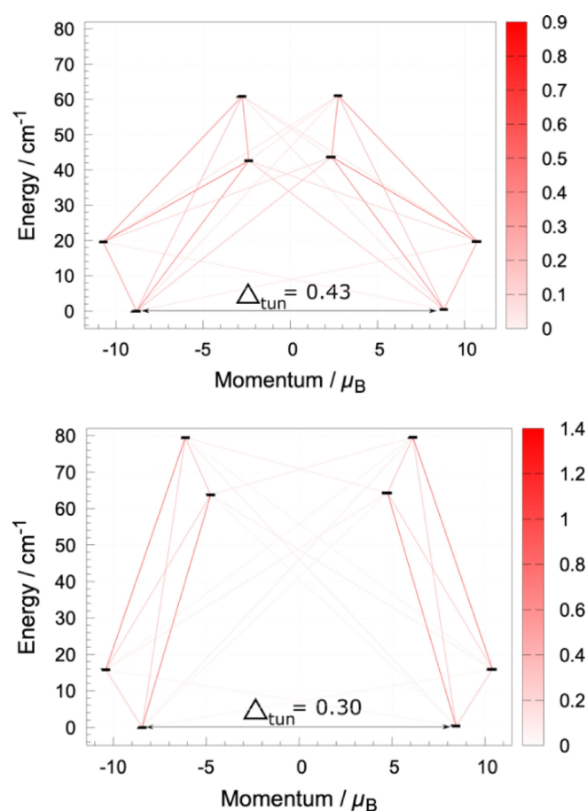
Figure 7. Blocking barrier for 1 as predicted by the two computational approaches employed. (top) the method using the relative energy between ^3\text{H} and ^7\text{H} terms of 20\text{ cm}^{-1} , J = -6.6\text{ cm}^{-1} ; (bottom) the Lines model (POLY_ANISO) with J = -7.0\text{ cm}^{-1} . Because of the significant value of tunnel splitting predicted by either method, the molecule is not a performant single-molecule magnet, in line with experimental evidence.
