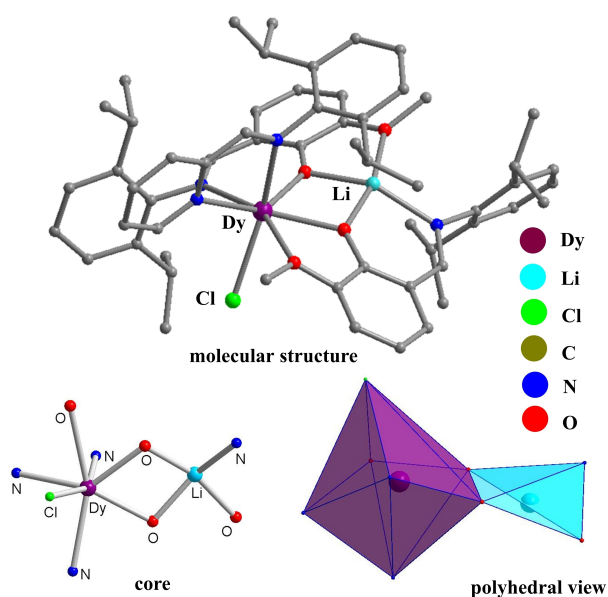
Figure 1. The molecular structure of the complex [Li(l)Dy(III)(L)(L NN•− )(Cl)]·tol ( 1 ·tol) and its core structure.
