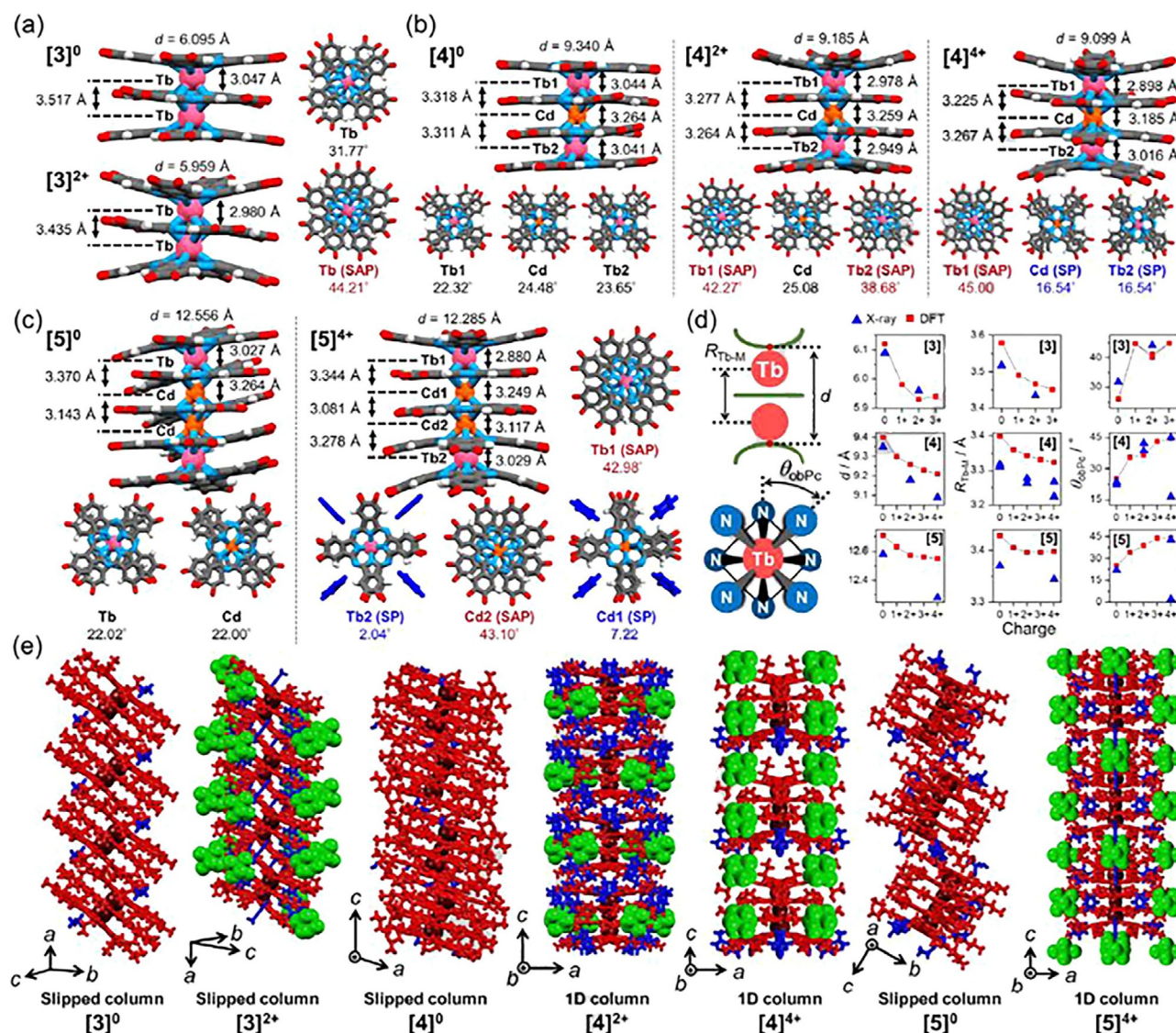
Figure 3. Crystal structures of (a) [3], (b) [4] and (c) [5]. The n -butoxy chains were omitted for clarity. (d) Charge dependence of the molecular length d , Tb-metal ion (Tb or Cd) distances R_{Tb-M} and stacking angle around metal ions \theta_{obPc} . (e) Packing structures of multiple-decker complexes. Red, green and blue parts represent multiple-decker units, counter anions ( SbCl_6 ) and solvent molecules, respectively.
